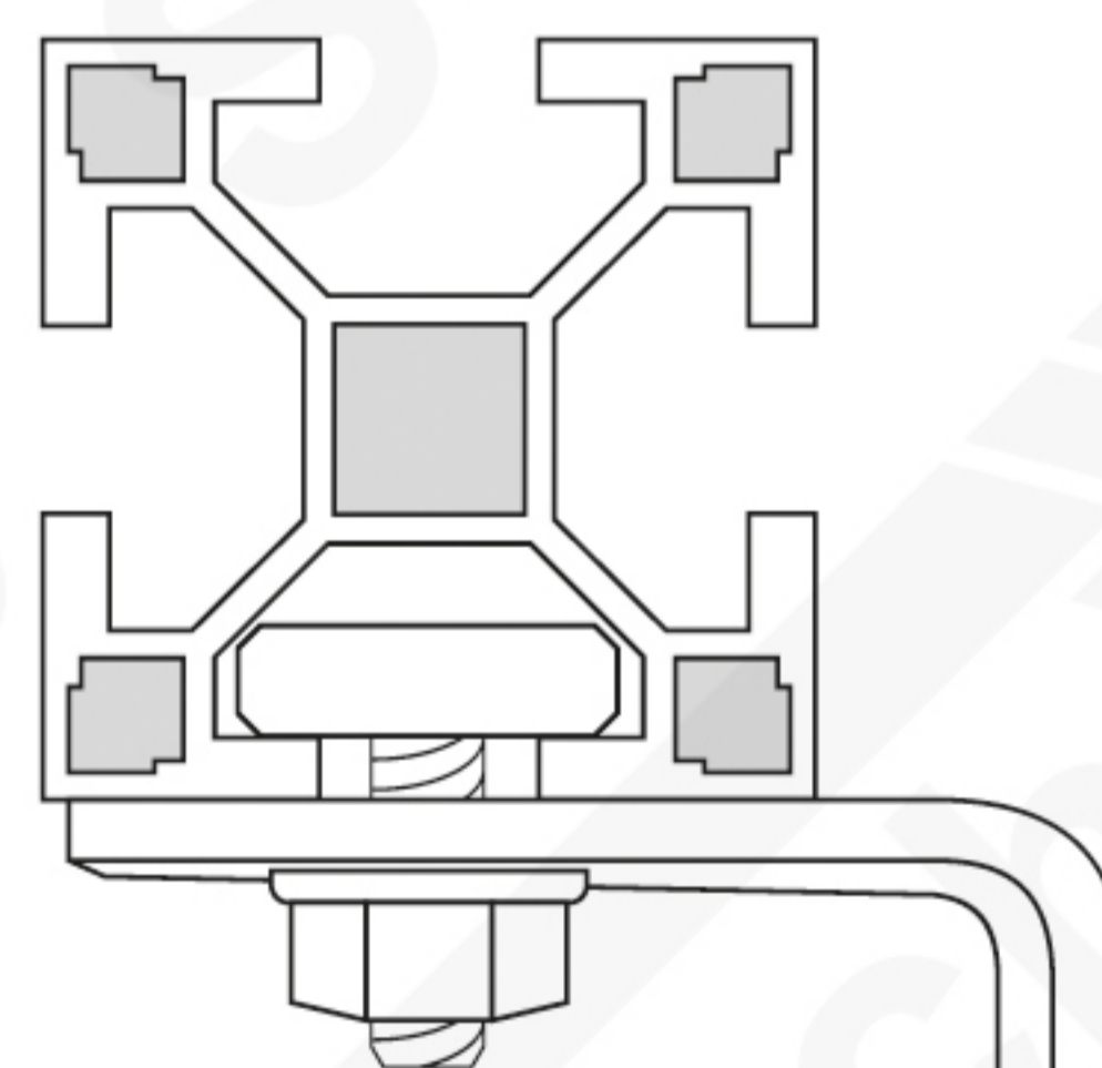
Dachhaken
