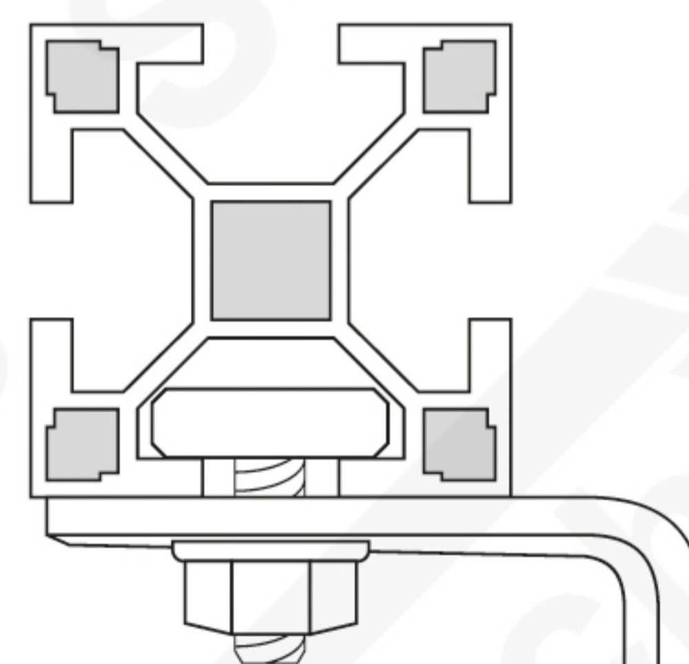
Dachhaken
